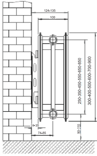
DF DOUBLE PANEL DOUBLE CONVECTOR
