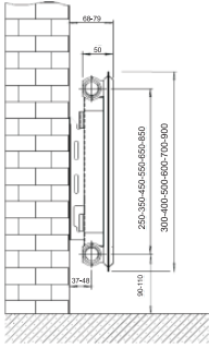
SF SINGLE PANEL SINGLE CONVECTOR
