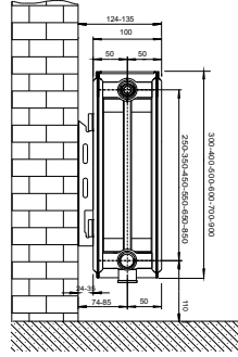
DS DOUBLE PANEL DOUBLE CONVECTOR
