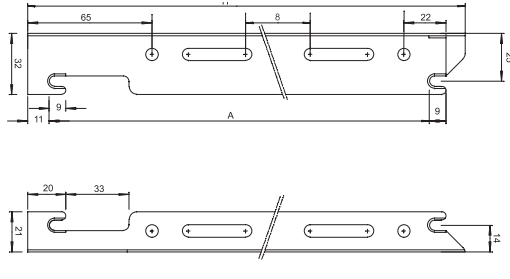
DF DOUBLE PANEL DOUBLE CONVECTOR
