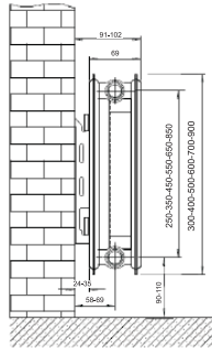
HF DOUBLE PANEL SINGLE CONVECTOR
